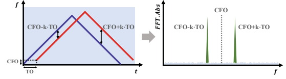
Figure 8: Coarse-grained estimation of CFO and TO.
